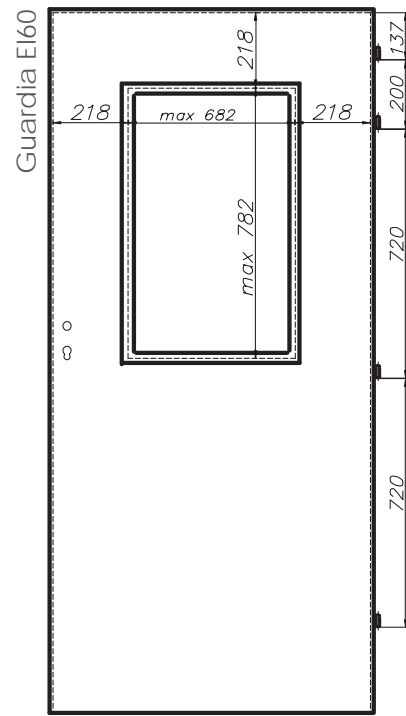
Door leaf thickness EI60 = 66 mm
