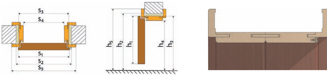
DIMENSIONS OF DOOR LEAF AND ADJUSTABLE DOOR FRAME (mm)
