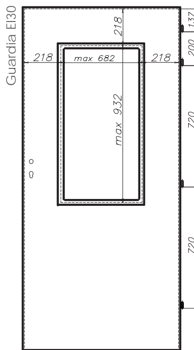
Door leaf thickness EI30 = 56 mm
