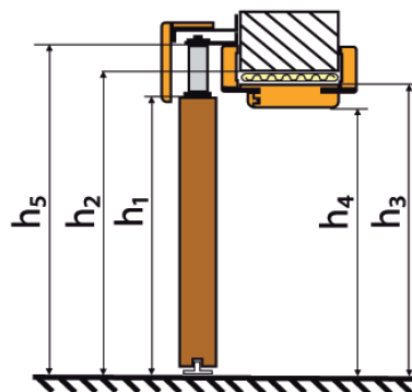
DIMENSIONS OF DOOR LEAF AND DOOR FRAME FOR ON-WALL SLIDING SYSTEM (mm)
